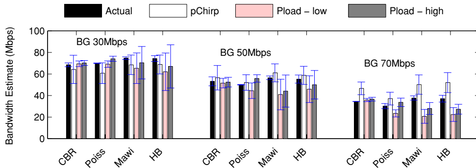
Figure 12: Augmenting to and validating pathload vs. pathchirp experiments from [17].
