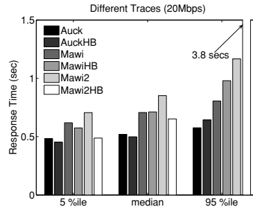
Figure 9: Simply generating “bursty” traffic is not enough.
