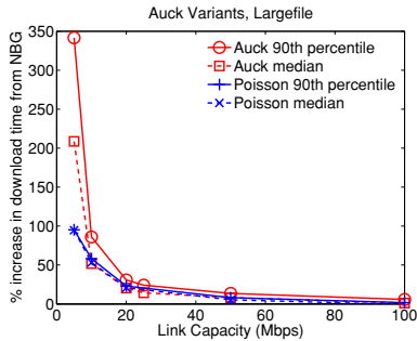
Figure 8: Varying link capacities.
